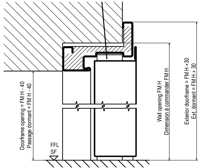
Vertical cross section Coupe verticale
