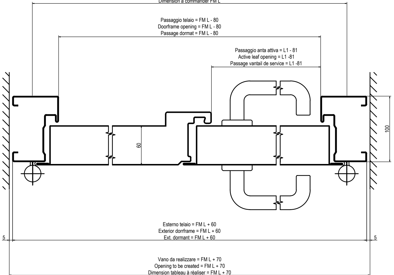
Foro muro FM L Wall opening FM L Dimension à commander FM L
