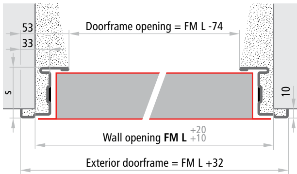
One-leaved doors Horizontal cross section
